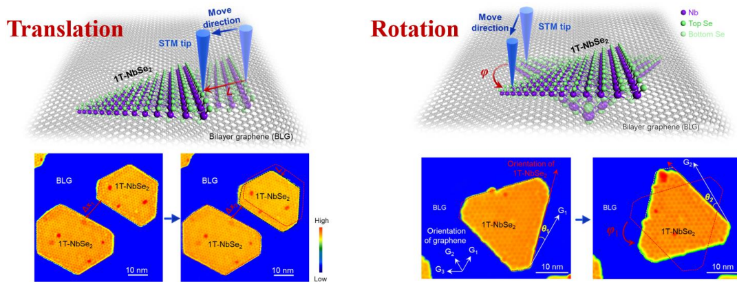
Figure 1. Controllable translation and rotation movement of NbSe 2 islands using STM manipulation technique.
